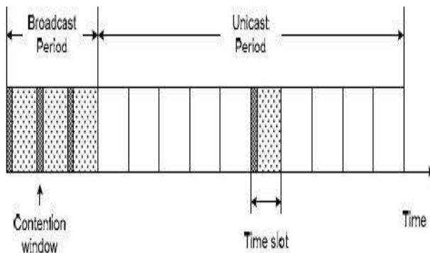
Fig 4: Frame architecture of Y-MAC [3]
