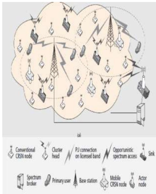
Fig 8: CRSN architecture [9]
