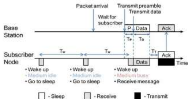
Fig 2: Preamble sampling in B-MAC
